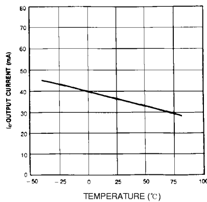
Fig. 12 CURRENT LIMITING
