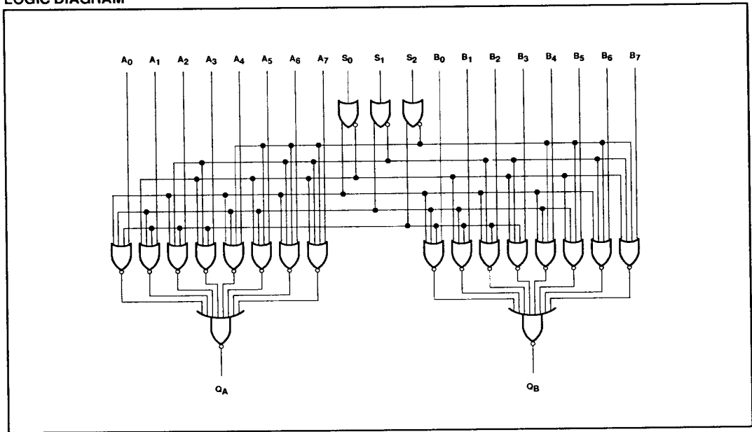
LOGIC DIAGRAM
