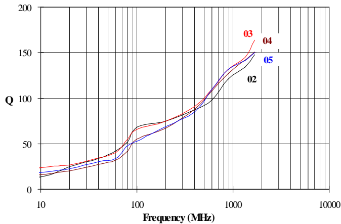
292A Series
