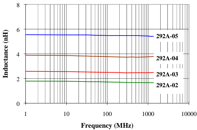
292A Series
