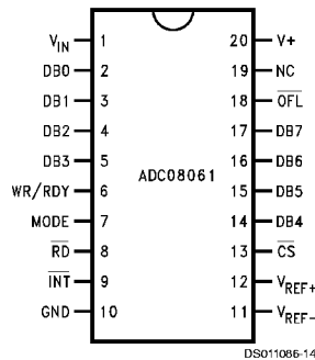
Dual-In-Line and Wide-Body Small-Outline Packages J20A, N20A or M20B
