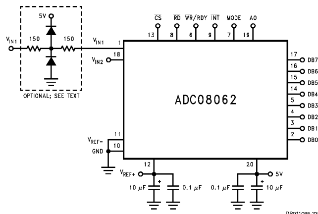
FIGURE 9. Typical Connection
