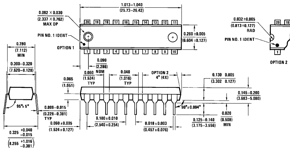
Dual-In-Line Package (N) Order Number ADC08061BIN, ADC08061CIN, ADC08062BIN or ADC08062CIN NS Package Number N20A
