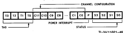
Data Output (DO) Word—ADC0858
