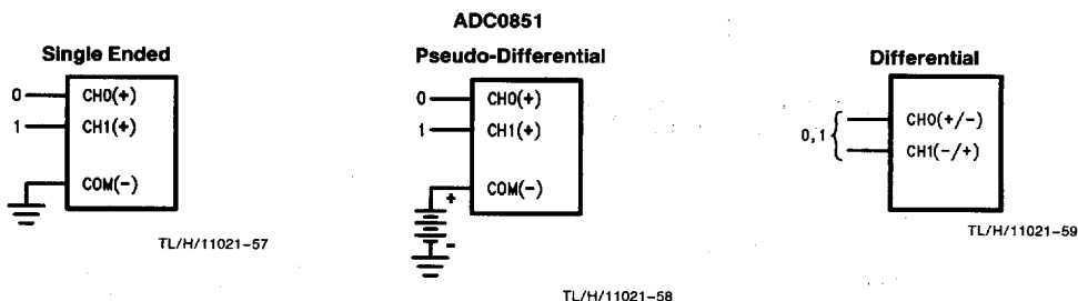
FIGURE 14. Analog Input Multiplexer Options for ADC0851
