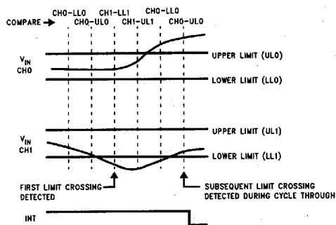
TL/H/11021-45 (Example: Lower limit of CH1 is crossed first. During cycle through, upper limit of CH0 is crossed)
