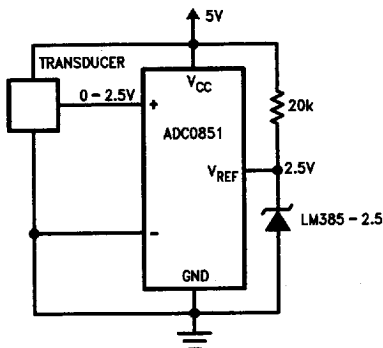
FIGURE 18. Absolute Input with 2.5V Input Voltage Span
