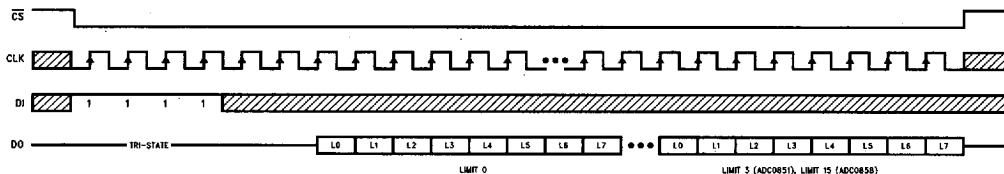
FIGURE 6. Timing Diagram for Read All Limits ADC0851/ADC0858
