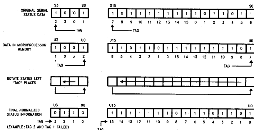
FIGURE 9. Status Bit Normalization
