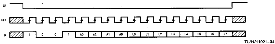
FIGURE 3. Timing Diagram for Write One Limit
