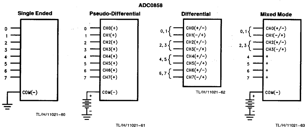
FIGURE 15. Analog Input Multiplexer Options for ADC0858
