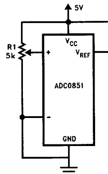
FIGURE 19. Single Channel Ratiometric Operation
