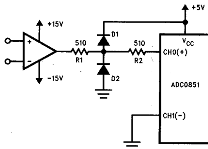
FIGURE 13. Over Voltage Protection of the Analog Inputs
