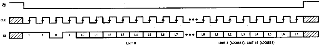
FIGURE 4. Timing Diagram for Write All Limits
