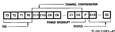
Data Output (DO) Word—ADC0858
