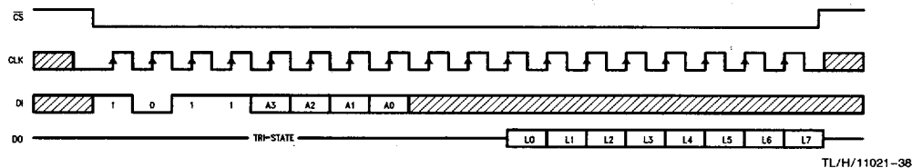
FIGURE 5. Timing Diagram for Read One Limit ADC0851/ADC0858
