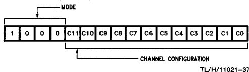
Data Input (DI) Word—ADC0851 or ADC0858
