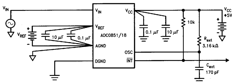
FIGURE 12. Recommended Connection for ADC0851 and ADC0858
