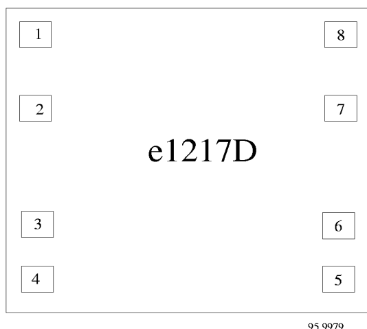
Figure 1. Chip size 1.06 mm x 1.02 mm Pad size: 112 \mu m x 112 \mu m (pad window 100 x 100)
