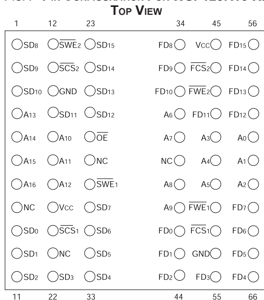
FIG. 1 PIN CONFIGURATION FOR WSF128K16-XHX AND WSF128K16-XH1X
