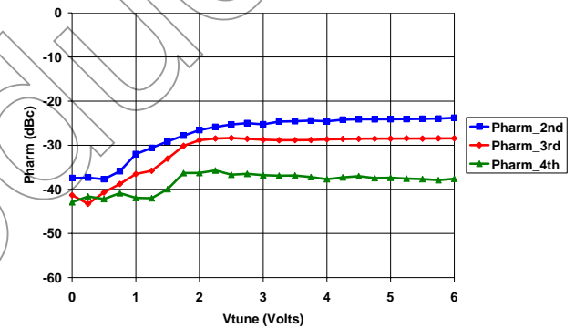
XQ1001-BD Harmonic Levels vs. Tuning Voltage
