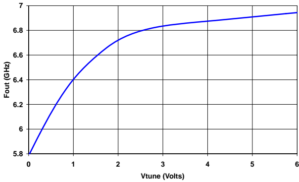
XQ1001-BD Output Frequency vs. Tuning Voltage
