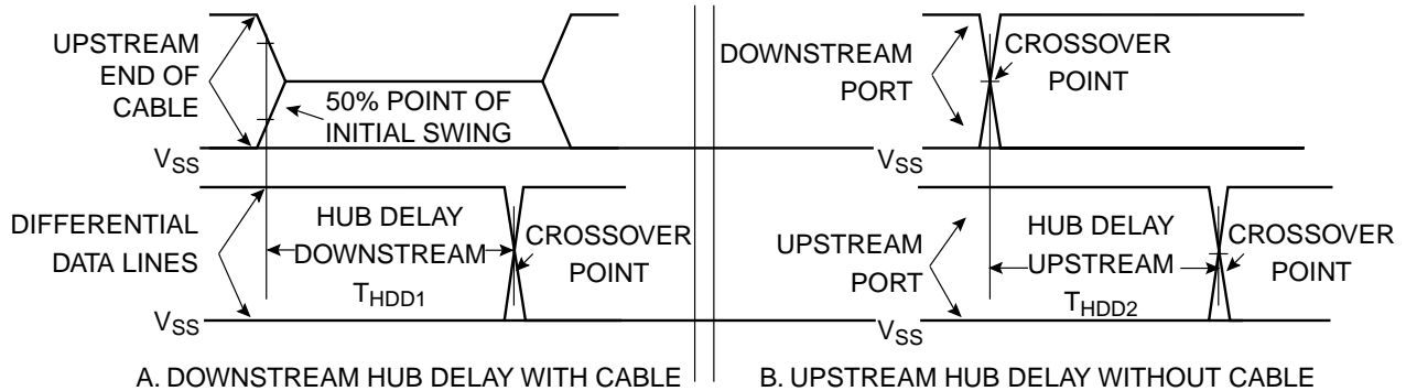
Figure 11. Hub Differential Delay, Differential Jitter, and SOP Distortion
