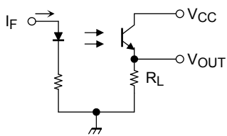
Note 3: Switching time measurement circuit and waveform
