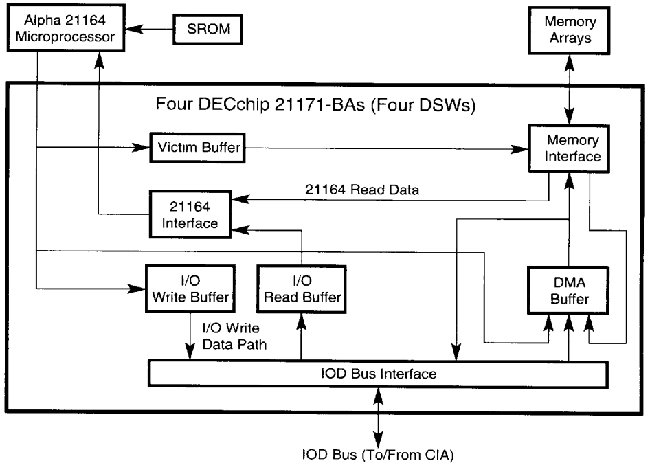
Figure 1-3 DSW Block Diagram
