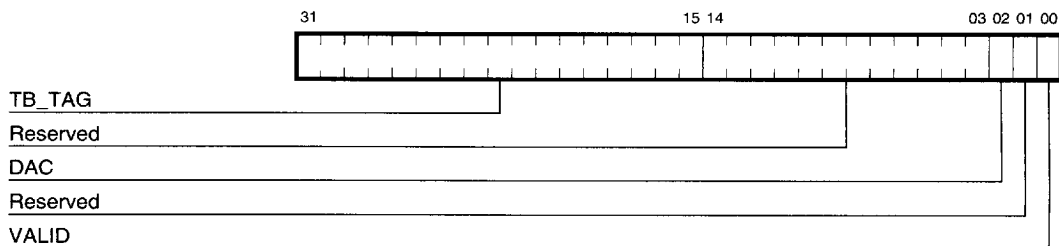
Figure 4–34 Translation Buffer Tag n Registers
