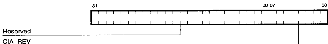
Figure 4–1 CIA Revision Register (87.4000.0080)
