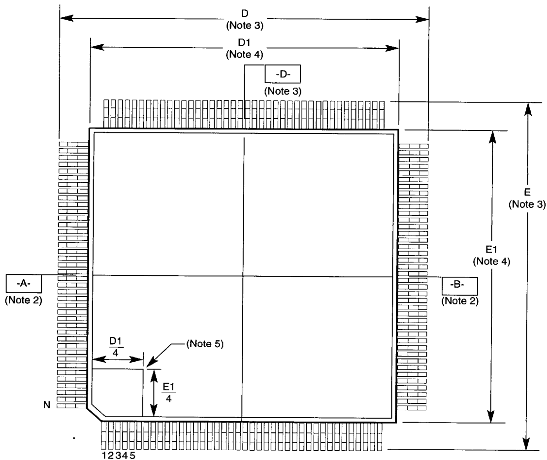
Figure 7-1 DECchip 21171-BA Package Dimensions
