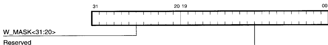
Figure 4-30 Window Mask Register n
