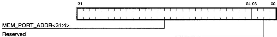
Figure 4–18 CIA Memory Port Status Register 0 (87.4000.8400)
