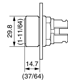
Non-Illuminated Maintained Push Button, Flush
