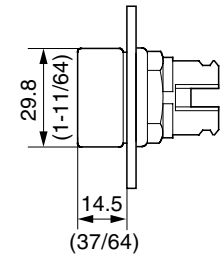
Non-Illuminated Momentary Push Button, Guarded
