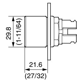
Non-Illuminated Momentary Push Button, Guarded
