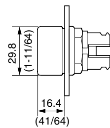
Pilot Light Standard
