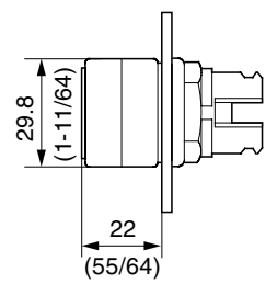
Illuminated Maintained Push Button, Flush
