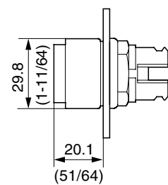
Non-Illuminated Reset Operator
