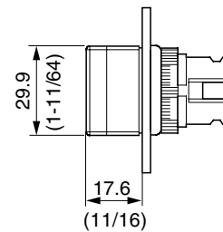
Key Operated Selector Switch Operator
