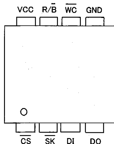
BR9040RFVM-W: MSOP8 BR9040RFV-W: SSOP8
