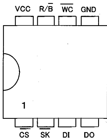
BR9040-W: DIP8
