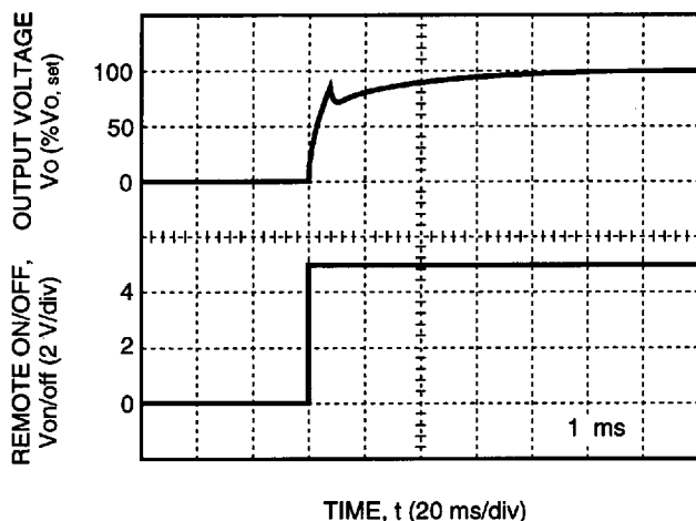
Figure 13. Typical Output Voltage Start-Up when Signal Applied to Remote On/Off
