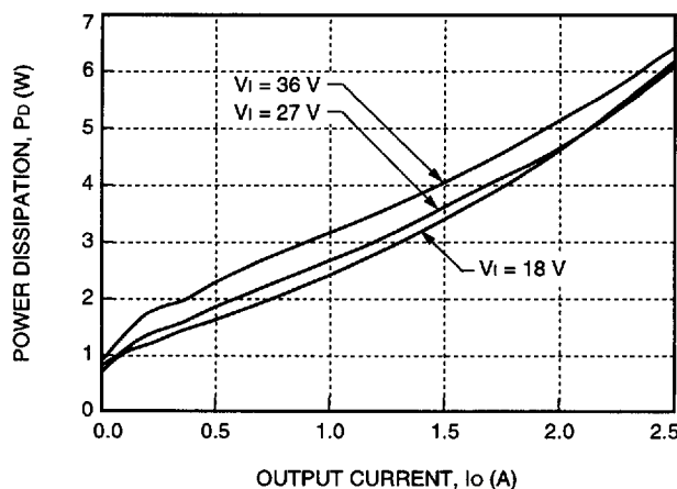
Figure 21. JC030B-M Power Dissipation vs. Output Current
