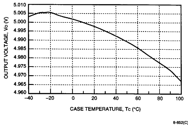
Figure 2. JC030A-M Typical Output Voltage Variation Over Ambient Temperature Range
