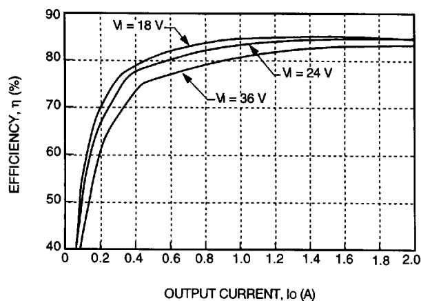
Figure 10. JC030C-M Typical Converter Efficiency vs. Output Current
