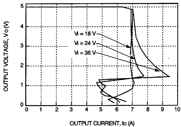
Figure 5. JC030A-M Typical Output Characteristics
