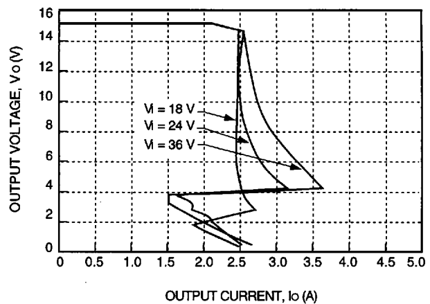
Figure 7. JC030C-M Typical Output Characteristics
