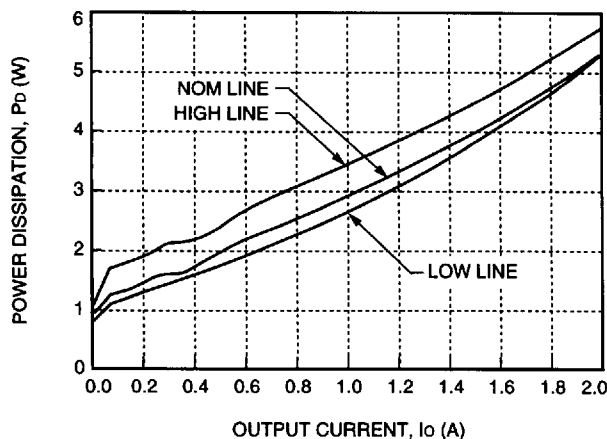
Figure 22. JC030C-M Power Dissipation vs. Output Current
