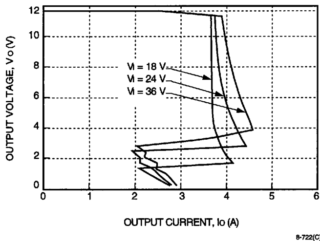
Figure 6. JC030B-M Typical Output Characteristics
