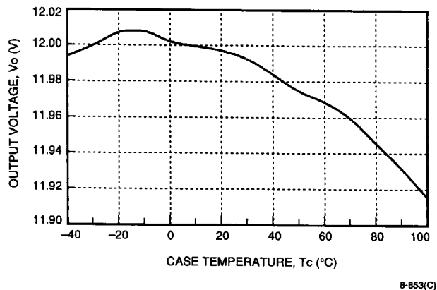
Figure 3. JC030B-M Typical Output Voltage Variation Over Ambient Temperature Range
