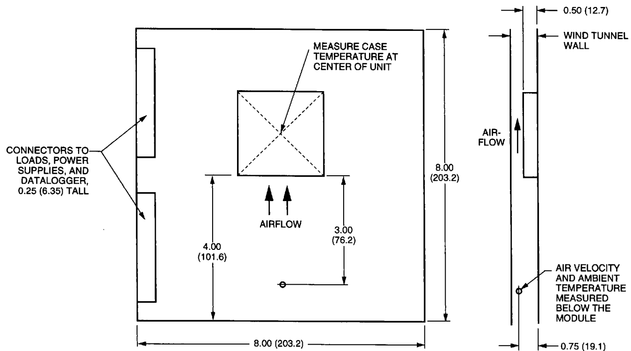
Figure 19. Thermal Test Setup
