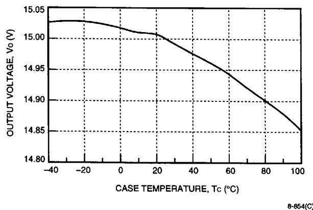
Figure 4. JC030C-M Typical Output Voltage Variation Over Ambient Temperature Range
