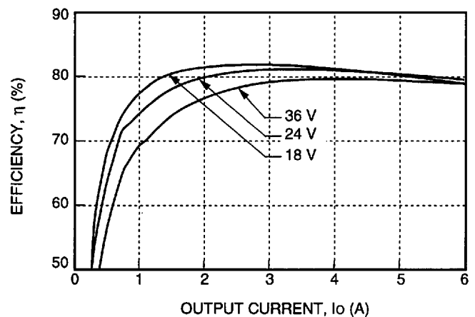
Figure 8. JC030A-M Typical Converter Efficiency vs. Output Current
