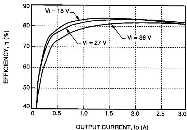
Figure 9. JC030B-M Typical Converter Efficiency vs. Output Current
