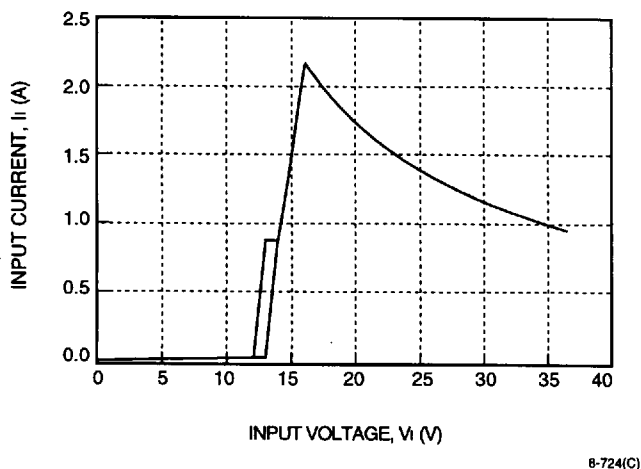
Figure 1. JC030-Series Typical Input Characteristic
