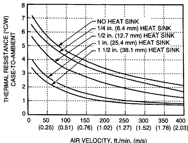
Figure 24. Case-to-Ambient Thermal Resistance vs. Air Velocity Curves; Either Orientation
