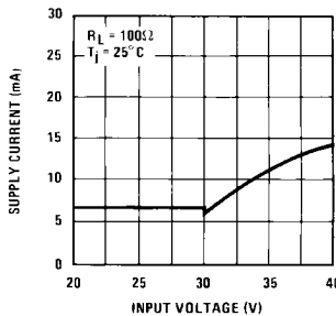
Overvoltage Supply Current
