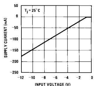
Reverse Supply Current
