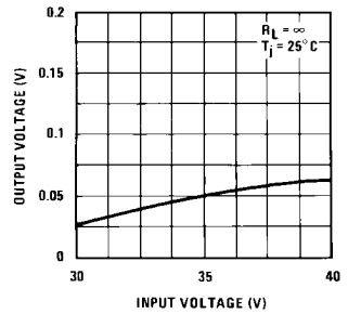
Output at Overvoltage
