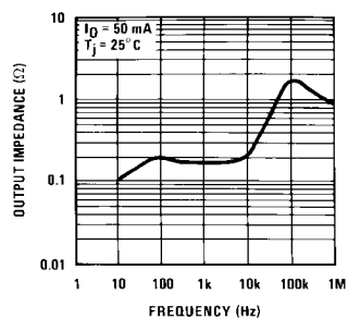
Output Impedance
