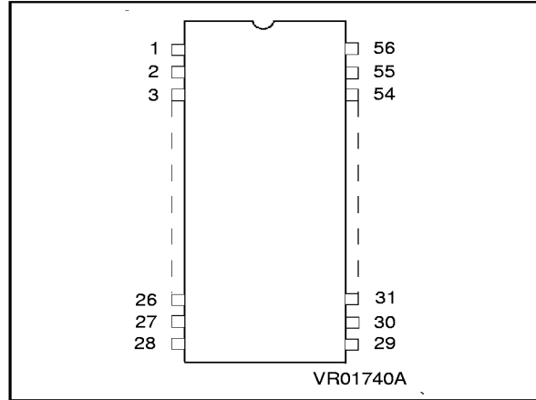
Figure 2. 56 Pin Shrink DIP Pinout
