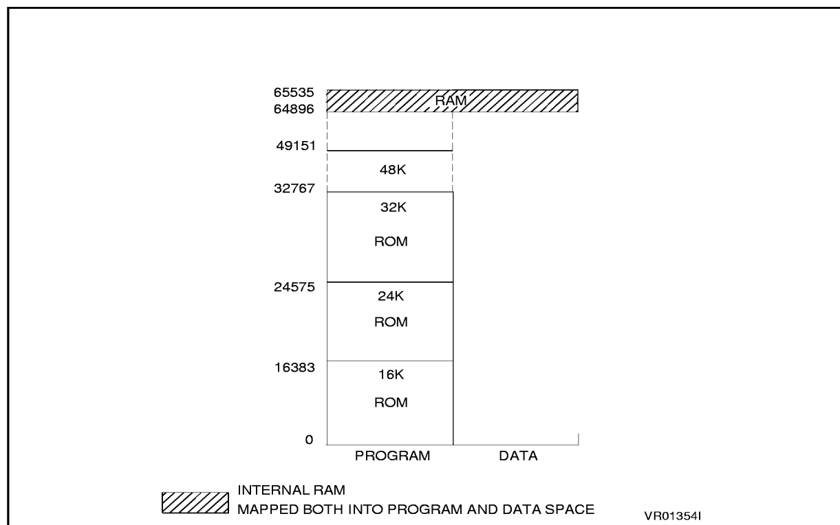
Figure 1-13. ST9291 Memory Map
