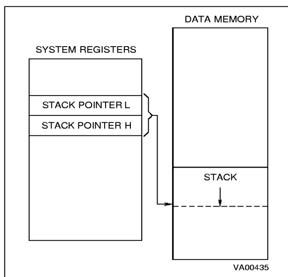
Figure 1-12. System and/or User Stack in Memory Stack Mode
