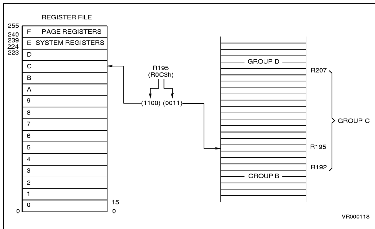
Figure 1-7. Addressing the Register File
