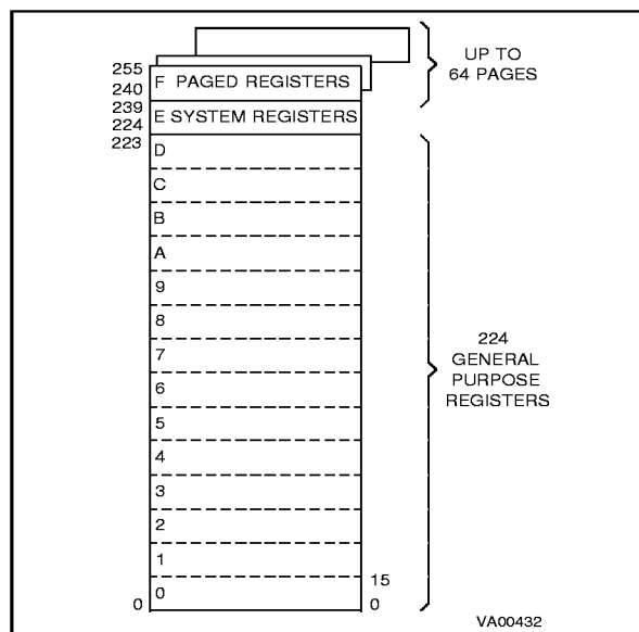
Figure 1-5. Register Grouping
