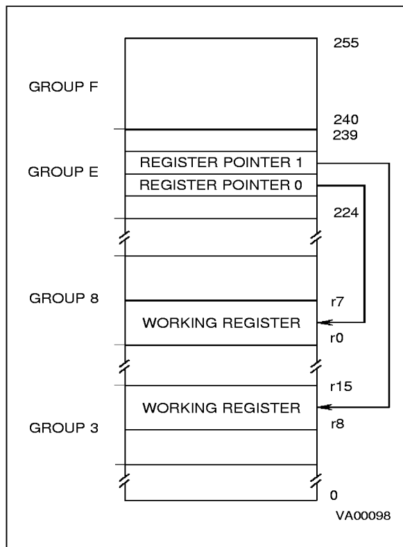
Figure 1-10. Double Register pointing Mode
