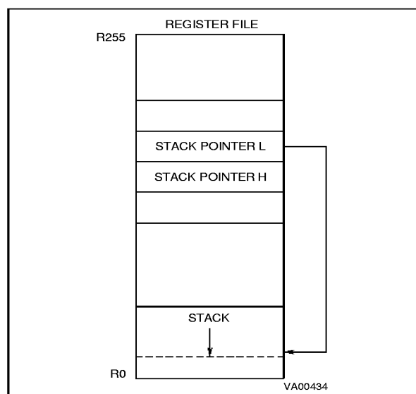
Figure 1-11. System and/or User Stack in Register Stack Mode
