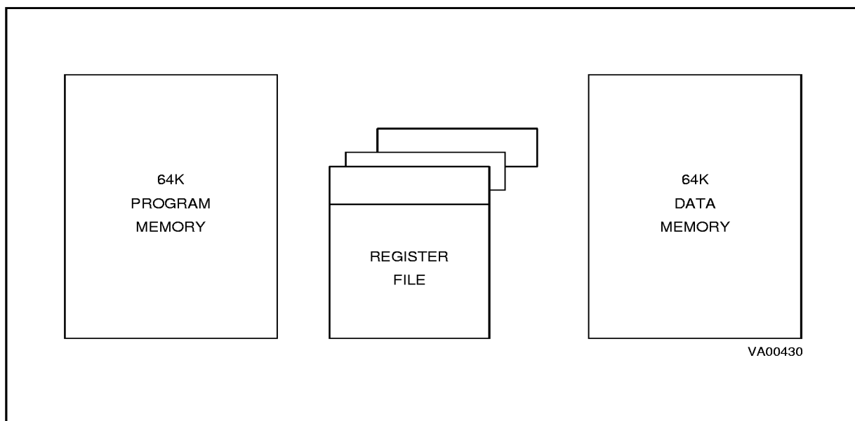
Figure 1-4. Address Spaces
