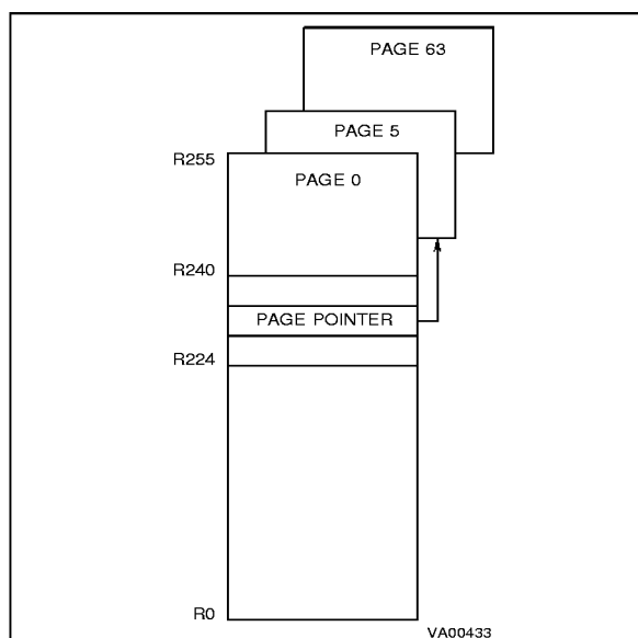
Figure 1-6. Page Pointer Configuration
