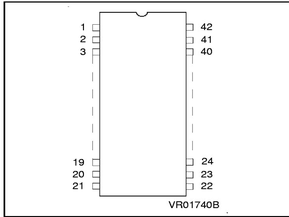
Figure 1. 42 Pin Shrink DIP Pinout
