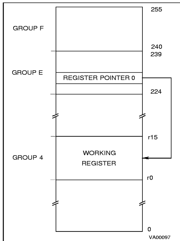
Figure 1-9. Single 16 Register pointing Mode
