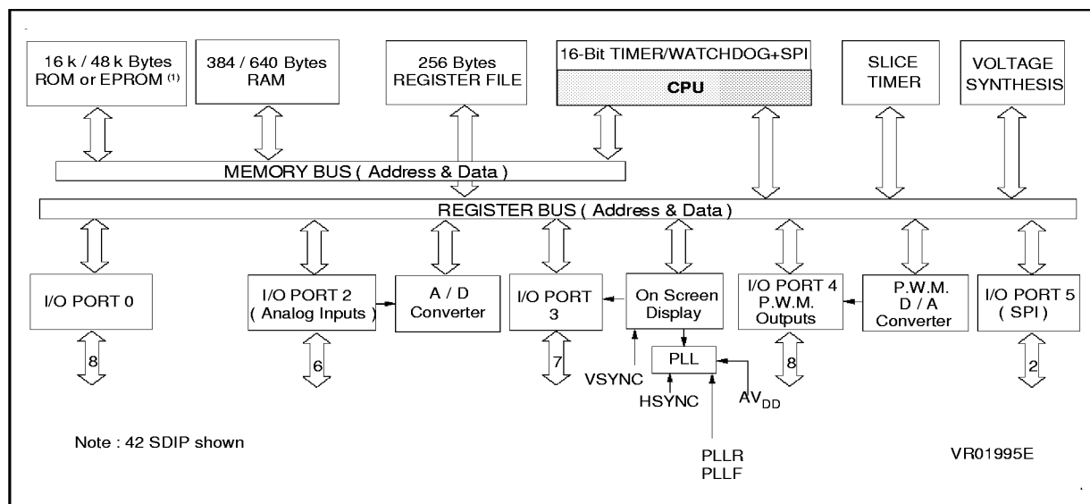
Figure 3. ST9291 Block Diagram
