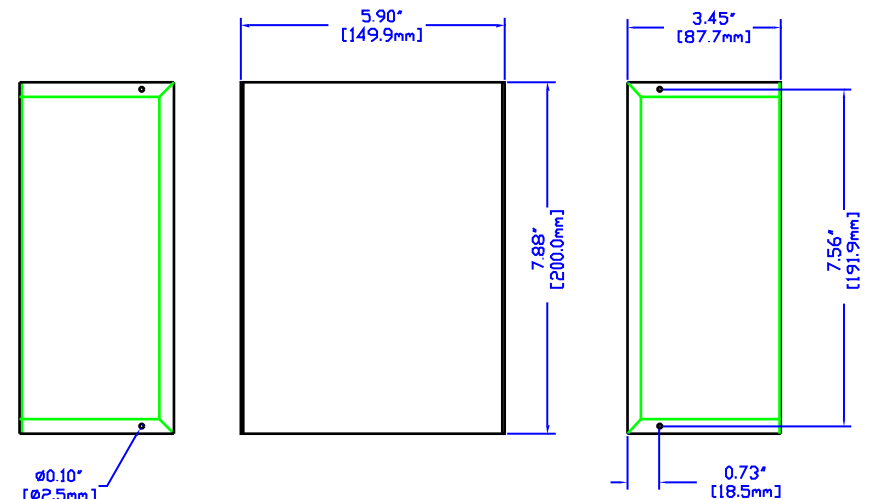
VIEW OF BASE (INSIDE)
