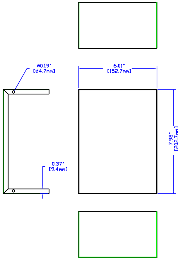
VIEW OF LID (INSIDE)
