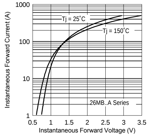
Fig. 2 - Forward Voltage Drop Characteristics Maximum Allowable Ambient T_a
