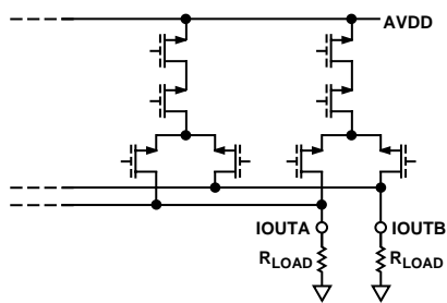
Figure 26. Equivalent Analog Output
