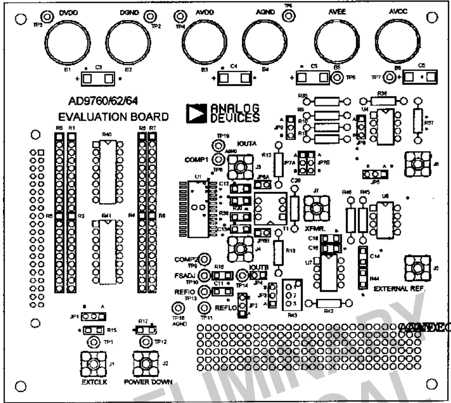
Figure 41. Silkscreen Layer—Top
