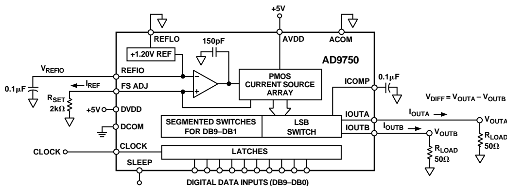
Figure 21. Functional Block Diagram
