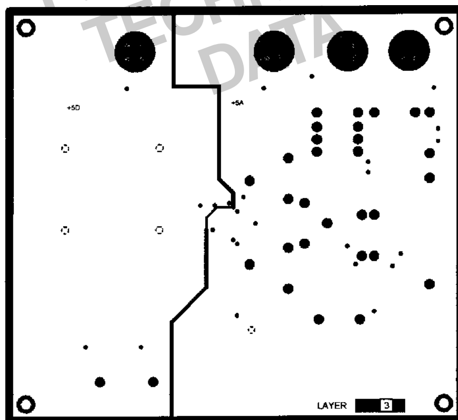
Figure 44. Power Plane PCB Layout (Layer 3)
