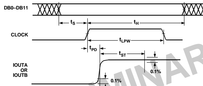
Figure 1. Timing Diagram
