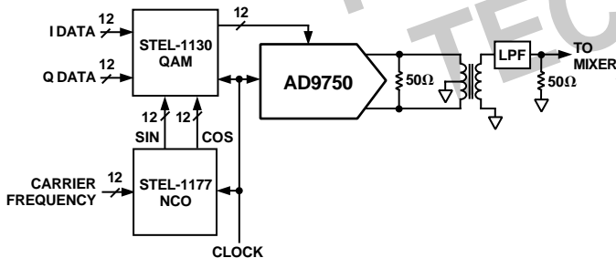
Figure 39. Digital QAM Architecture
