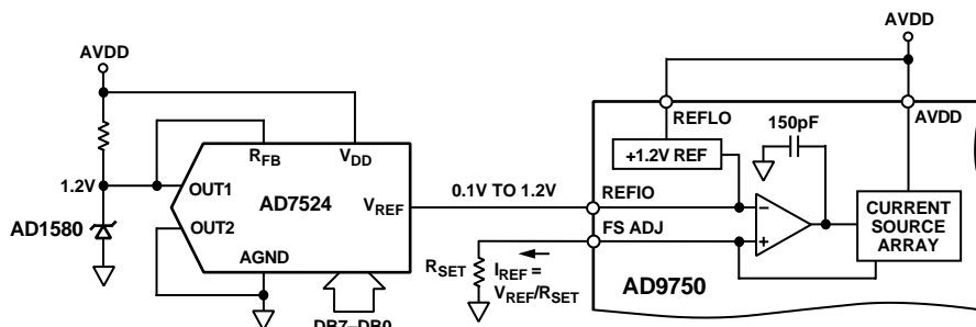
Figure 24. Single-Supply Gain Control Circuit
