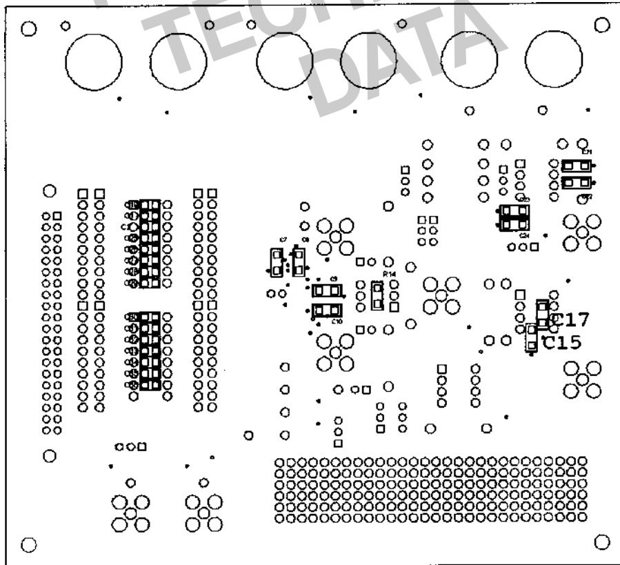
Figure 46. Silkscreen Layer—Bottom
