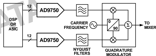
Figure 37. Typical Analog QAM Architecture
