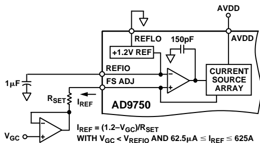
Figure 25. Dual-Supply Gain Control Circuit
