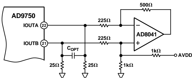
Figure 33. Single-Supply DC Differential Coupled Circuit
