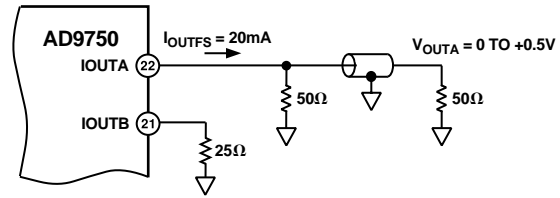
Figure 34. 0\text{ V} to +0.5\text{ V} Unbuffered Voltage Output
