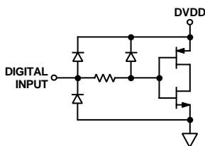
Figure 27. Equivalent Digital Input
