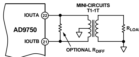
Figure 31. Differential Output Using a Transformer
