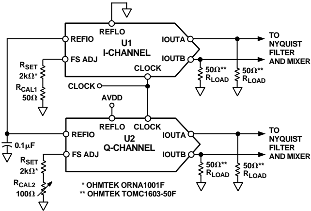
Figure 38. Baseband QAM Implementation Using Two AD9750s
