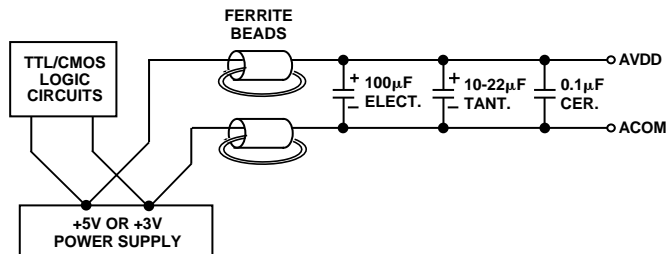
Figure 36. Differential LC Filter for Single +5 V or +3 V Applications
