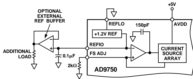
Figure 22. Internal Reference Configuration
