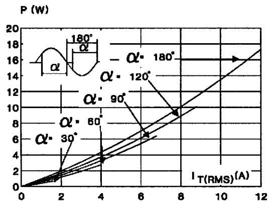
Fig. 1 : Maximum RMS power dissipation versus RMS on-state current ( F = 60\text{Hz} ). (Curves are cut off by (di/dt)_c limitation)
