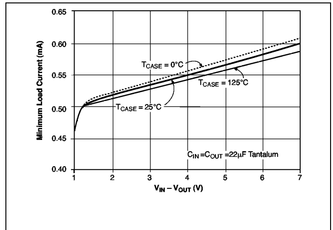
Minimum Load Current vs V_{IN} - V_{OUT}
