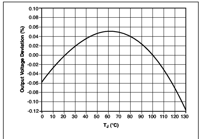
Reference Voltage vs. Temperature
