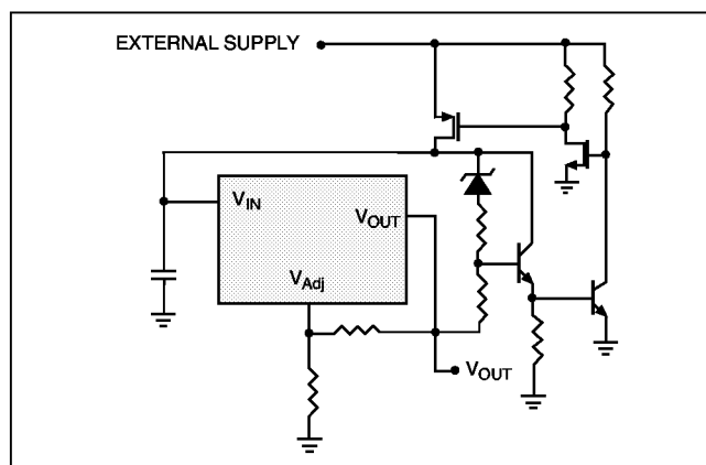
Figure 2: Short Circuit Protection Circuit for High Voltage Application.
