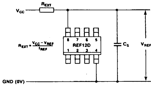
Fig.3 Connection diagram
