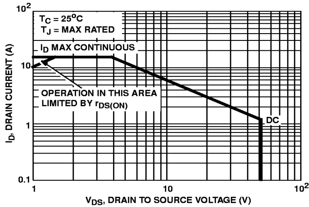
FIGURE 3. FORWARD BIAS SAFE OPERATING AREA
