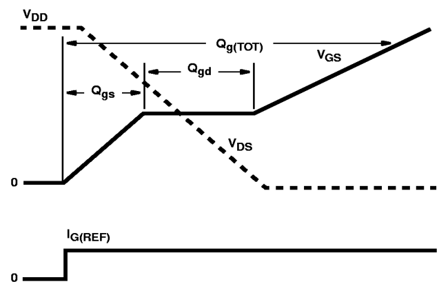
FIGURE 18. GATE CHARGE WAVEFORMS
