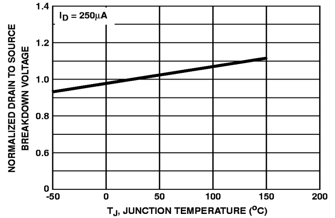
FIGURE 10. NORMALIZED DRAIN TO SOURCE BREAKDOWN VOLTAGE vs JUNCTION TEMPERATURE
