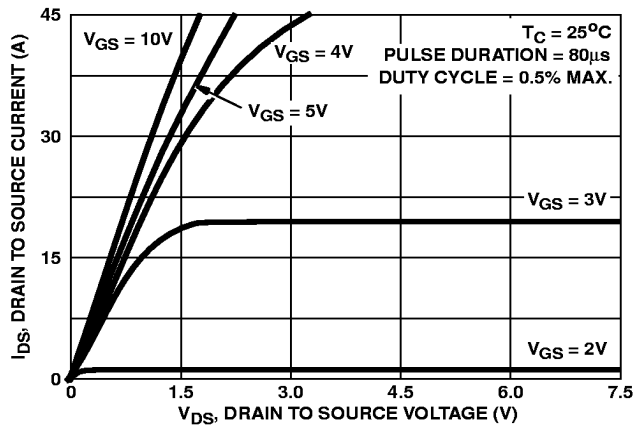
FIGURE 5. SATURATION CHARACTERISTICS
