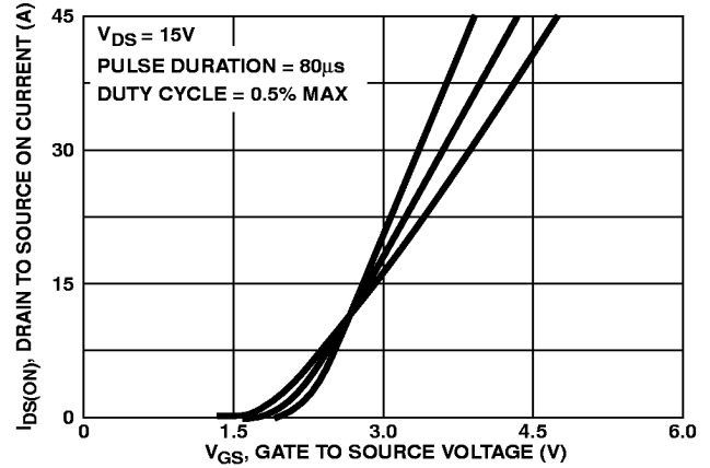
FIGURE 6. TRANSFER CHARACTERISTICS
