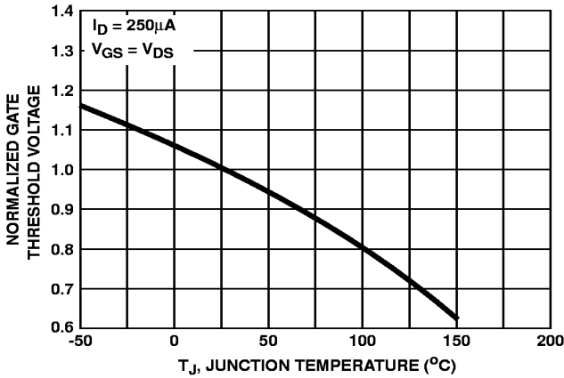
FIGURE 9. NORMALIZED GATE THRESHOLD vs JUNCTION TEMPERATURE
