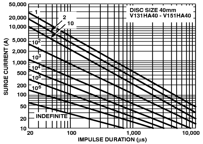
FIGURE 6. SURGE CURRENT RATING CURVES FOR V131HA40 - V151HA40
