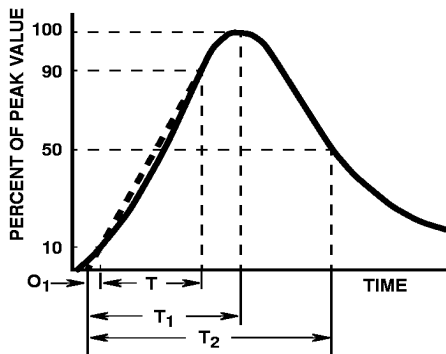
FIGURE 2. PEAK PULSE CURRENT WAVEFORM
