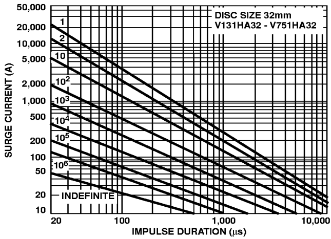
FIGURE 5. SURGE CURRENT RATING CURVES FOR V131HA32 - V751HA32
