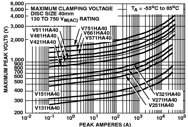
FIGURE 4. CLAMPING VOLTAGE FOR V131HA40 - V751HA40
