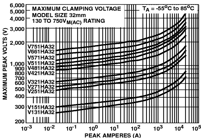
FIGURE 3. CLAMPING VOLTAGE FOR V131HA32 - V751HA32
