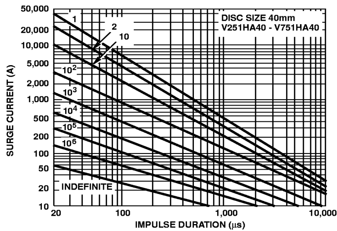
FIGURE 7. SURGE CURRENT RATING CURVES FOR V251HA40 - V751HA40
