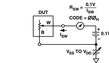
Test Circuit 8. Incremental ON Resistance
