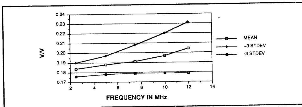
FIGURE 4c: Hysteresis Gain
