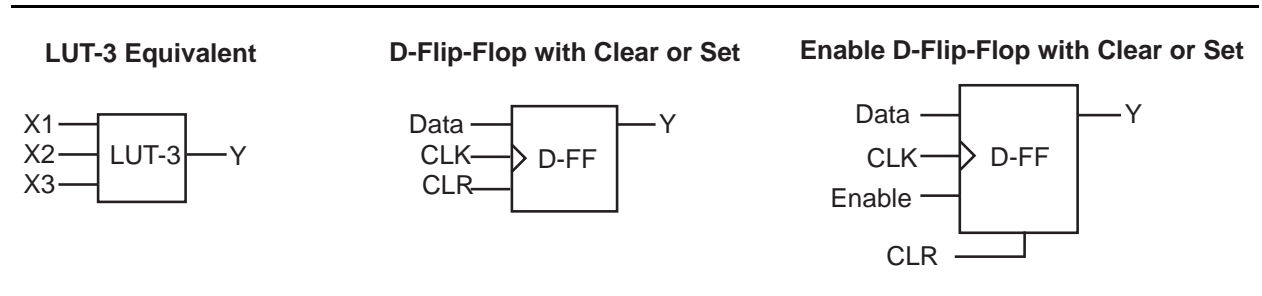
Figure 1-4 • VersaTile Configurations
