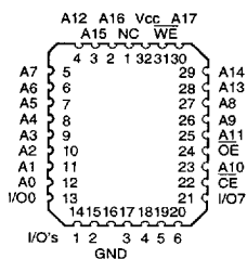
PLCC (1) Top View
