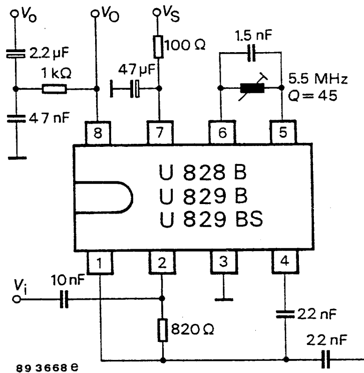
Figure 4. Test circuit
