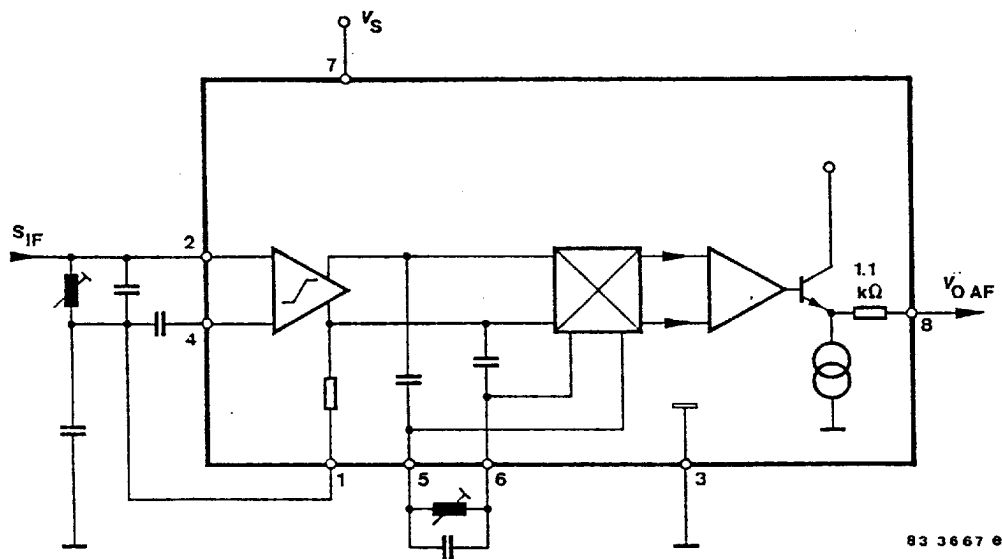
Figure 1. Block diagram U828B
