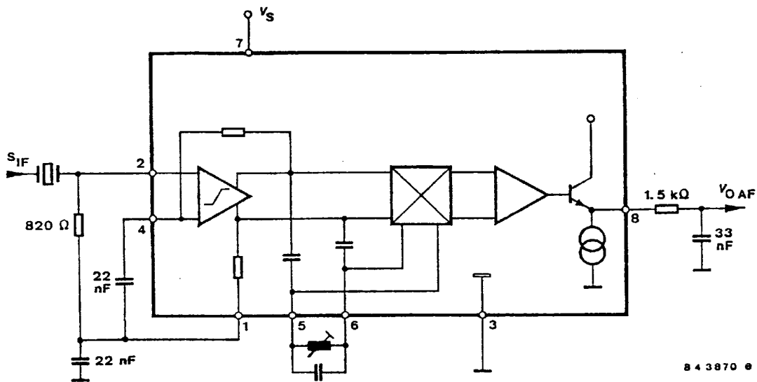
Figure 2. Block diagram U829B
