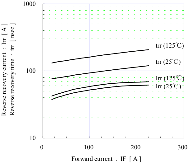
Reverse recovery characteristics (typ.) Vcc=300V, VGE=±15V, Rg=24Ω
