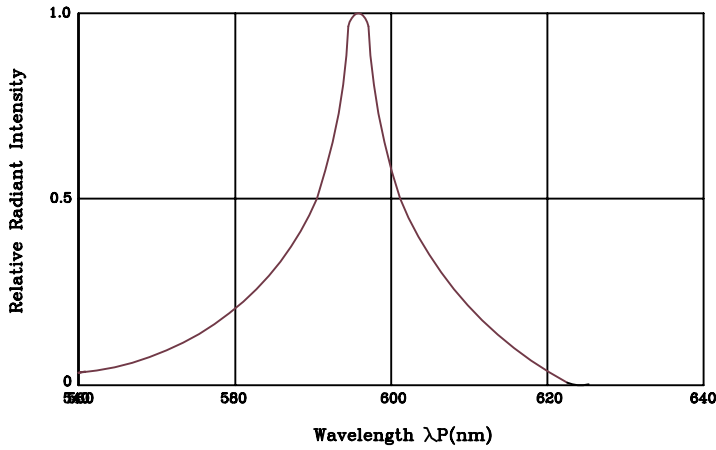
SPECTRAL DISTRIBUTION
