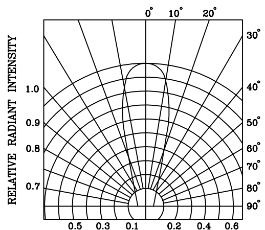
RADIATION DIAGRAM
