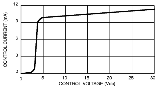
CONTROL CURRENT VS CONTROL VOLTAGE FIGURE 1
