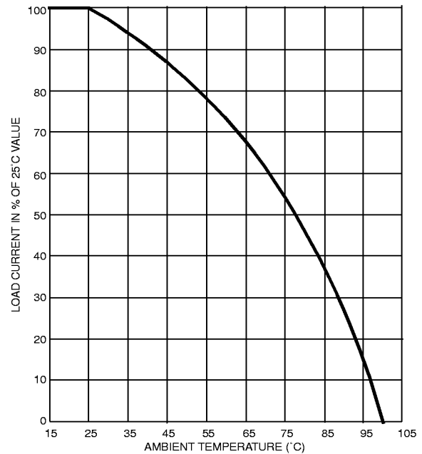
MAXIMUM LOAD CURRENT VS TEMPERATURE FIGURE 3
