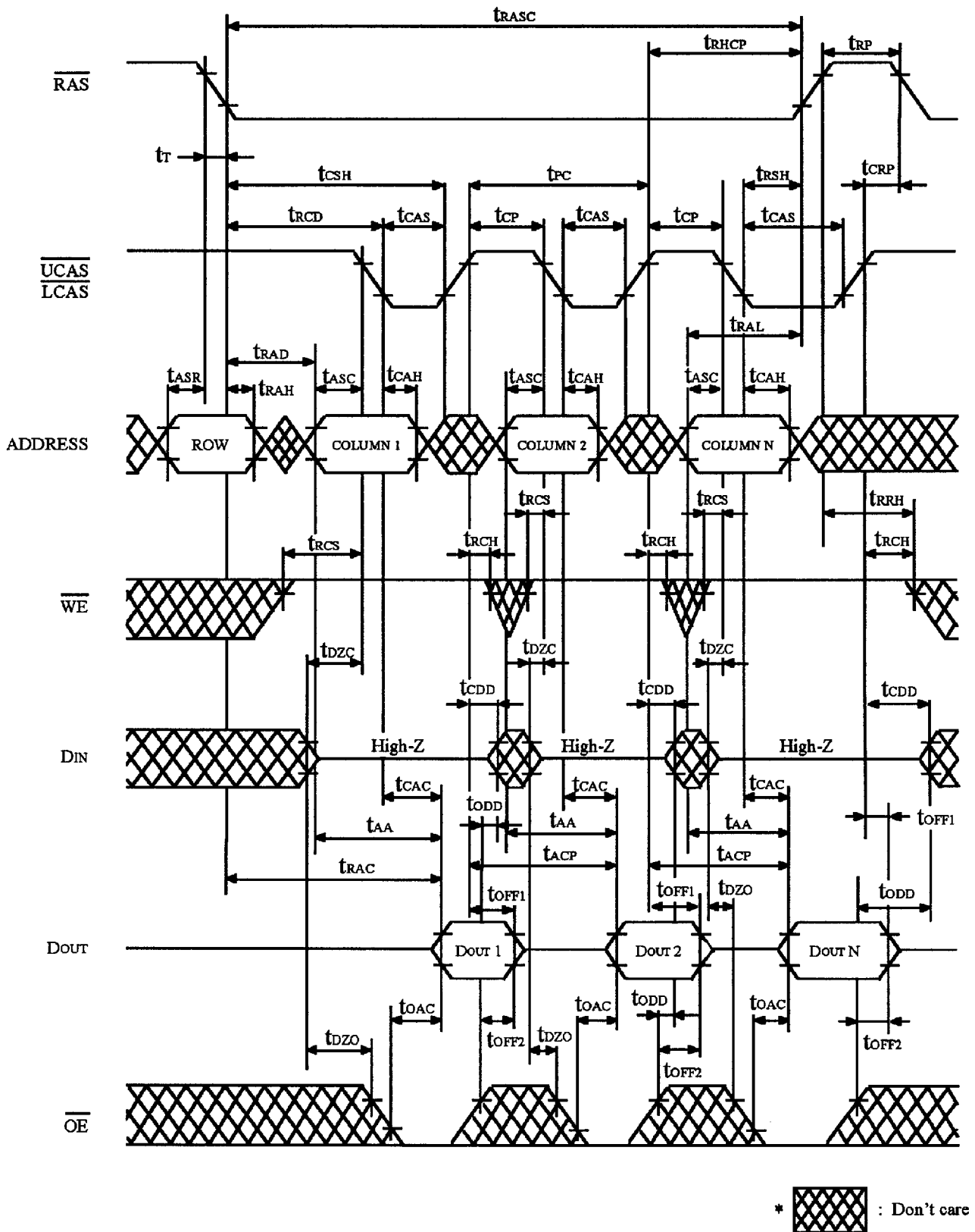
FIGURE 6. FAST PAGE MODE READ CYCLE
