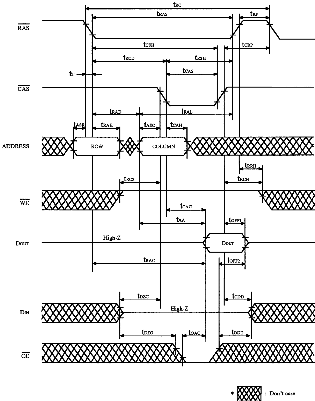
FIGURE 1. READ CYCLE
