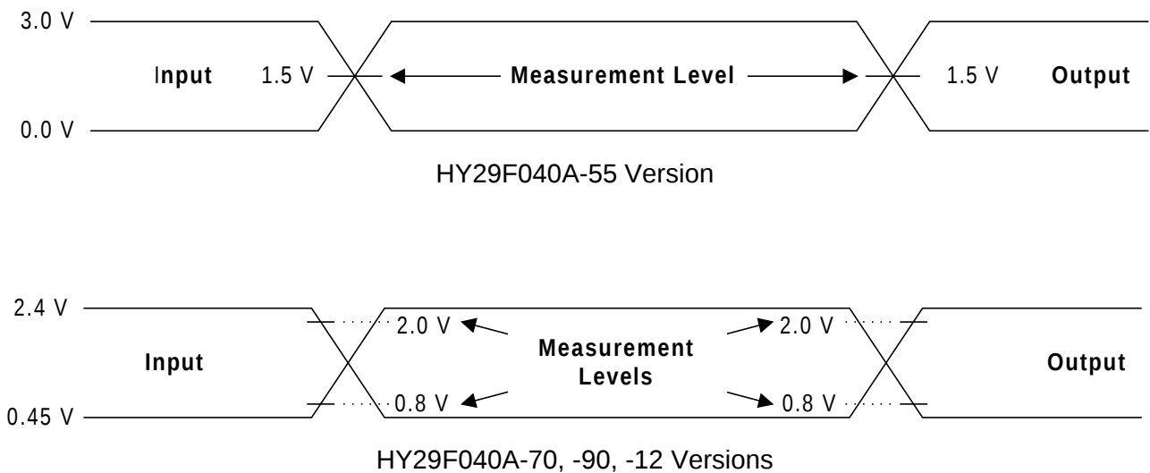
Figure 11. Input Waveforms and Measurement Levels
