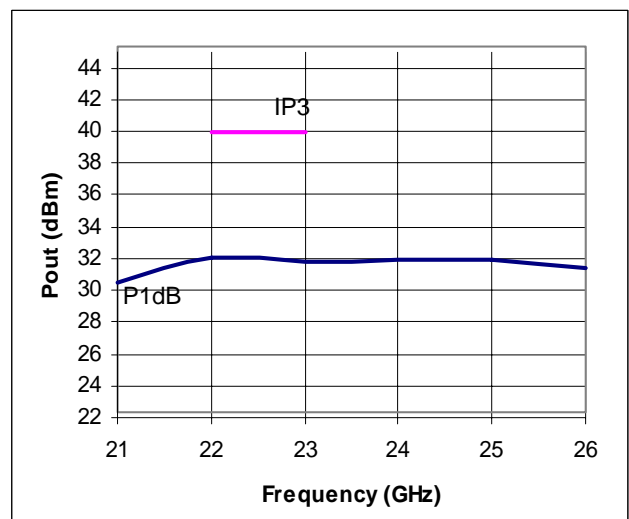
Two tone test with 18 dBm / tone
