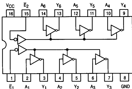
LOGIC DIAGRAM
