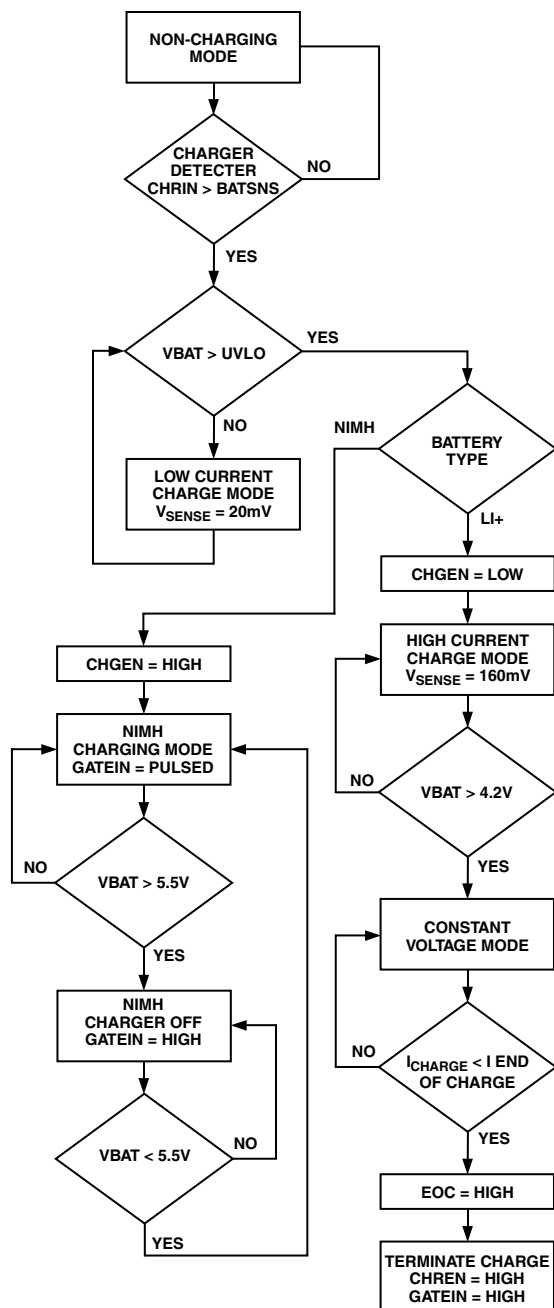
Figure 5. Battery Charger Flow Chart
