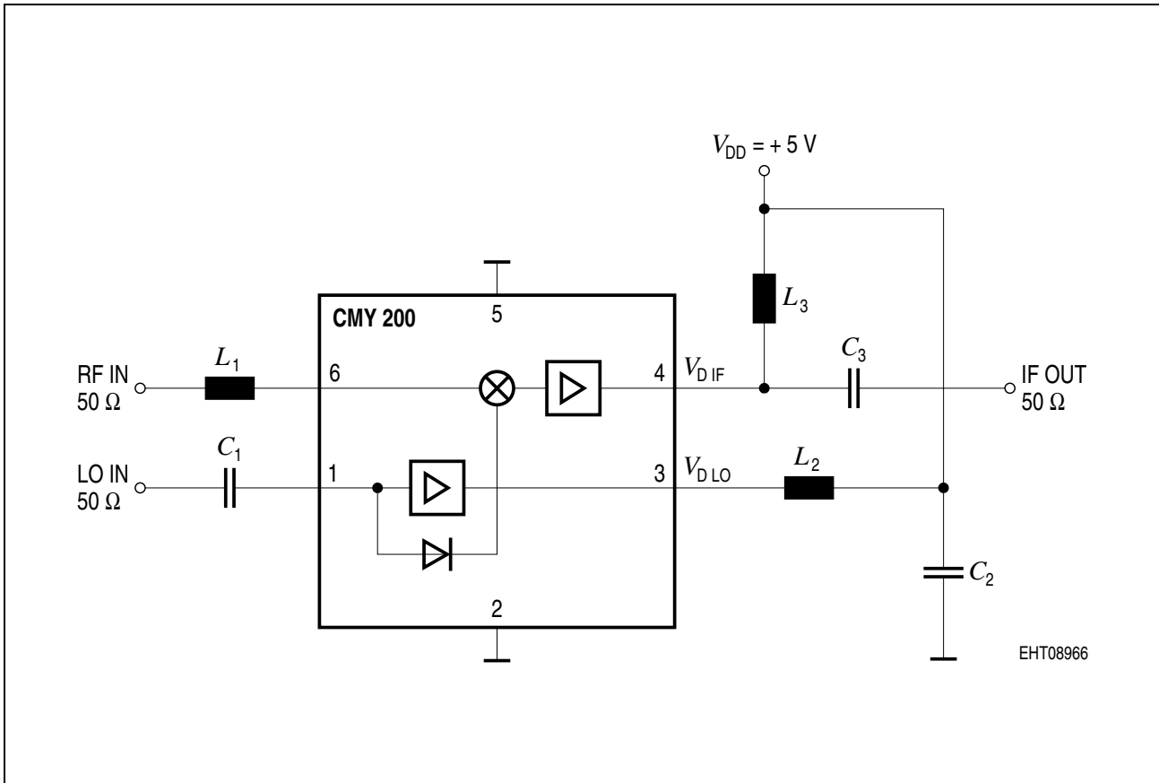
Figure 1 Test Circuit
