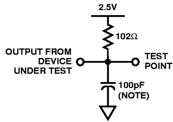
BUSY, CBRQ LOAD CIRCUIT
