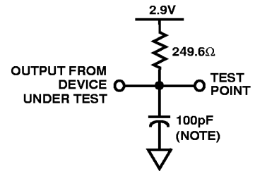
BPRO, BREQ LOAD CIRCUIT
