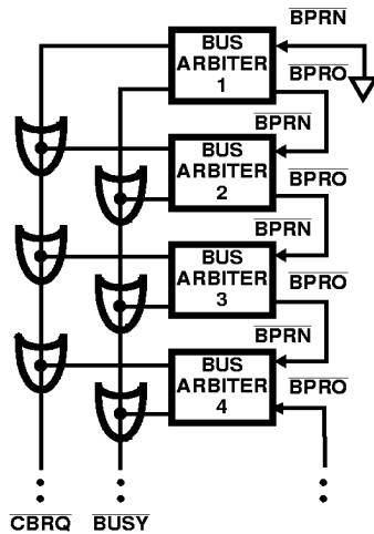
FIGURE 3. SERIAL PRIORITY RESOLVING
