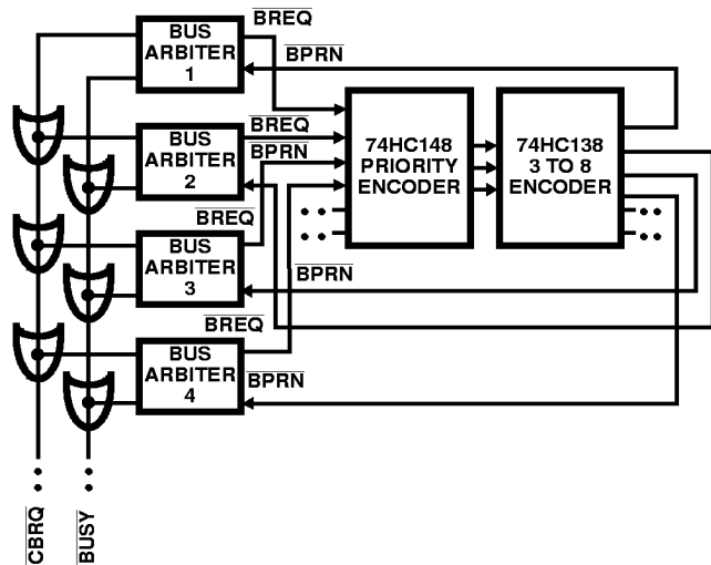
FIGURE 1. PARALLEL PRIORITY RESOLVING TECHNIQUE
