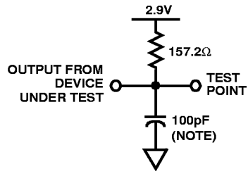
AEN LOAD CIRCUIT
