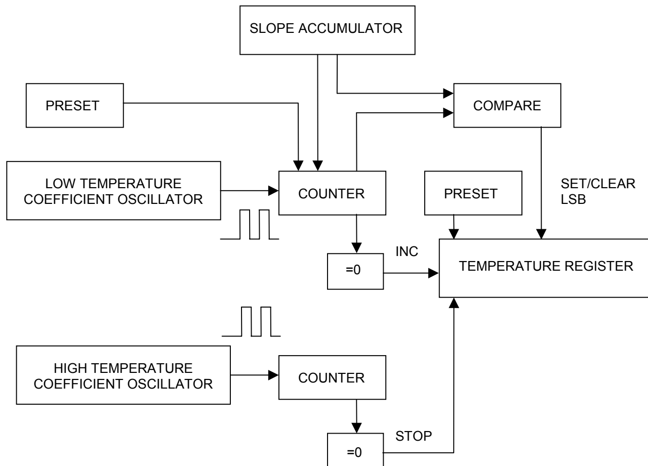
Figure 2. TEMPERATURE MEASURING CIRCUITRY
