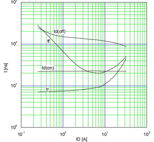
Typical Switching Characteristics vs. I D t=f(I_D):V_{cc}=300V, V_{GS}=10V, R_G=10\Omega
