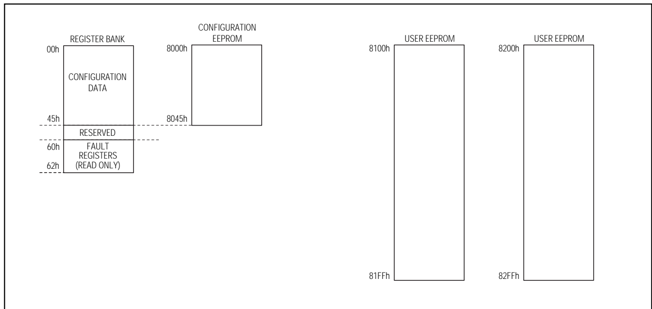
Figure 8. Memory Map
