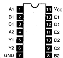
NTE74LS260, NTE74S260 14-Lead DIP, See Diag. 247 Dual 5-Input NOR Gate
