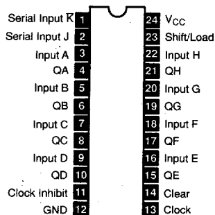
NTE74199 24-Lead DIP, See Diag. 252 8-Bit Bidirectional Universal Shift Register
