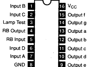
NTE74LS248, NTE74249, NTE74LS249 16-Lead DIP, See Diag. 249 BCD-to-Seven-Segment Decoder/Driver
