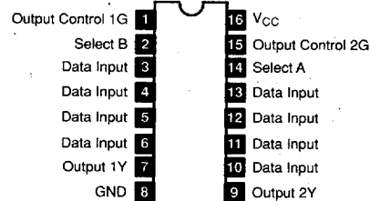
NTE74LS253 16-Lead DIP, See Diag. 249 Dual Data Selector/Multiplexer w/3-State Outputs
