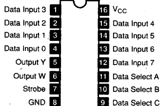
NTE74251, NTE74LS251, NTE74S251 16-Lead DIP, See Diag. 249 Data Selector/Multiplexer w/True & Inverted 3-State Outputs
