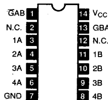
NTE74LS242, NTE74LS243 14-Lead DIP, See Diag. 247 Quad Bus Transceiver w/3-State Outputs
