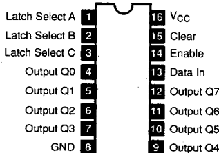
NTE74HC259, NTE74LS259 16-Lead DIP, See Diag. 249 8-Bit Addressable Latch
