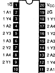
NTE74C240, NTE74HC240, NTE74HCT240, NTE74LS240, NTE74LS241, NTE74C244, NTE74HC244, NTE74HCT244, NTE74LS244 20-Lead DIP, See Diag. 294 Octal Buffer/Line Driver/Receiver w/3-State Outputs
