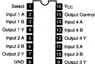
NTE74HC257, NTE74LS257, NTE74S257, NTE74LS258, NTE74S258 16-Lead DIP, See Diag. 249 Quad Data Selector/Multiplexer w/3-State Outputs
