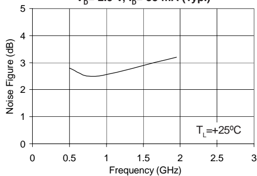
Noise Figure vs. Frequency V D = 2.9 V, I D = 35 mA (Typ.)
