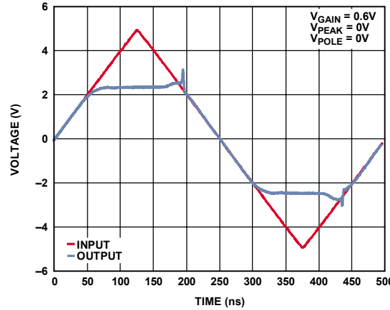
Figure 10. Overdrive Recovery
