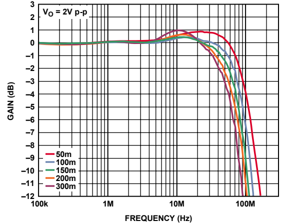
Figure 8. Equalized Frequency Response for Various Cable Lengths
