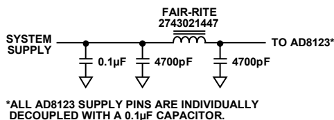
Figure 30. Power Supply Filter
