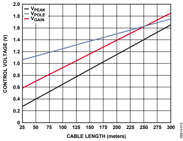
Figure 17. Recommended Settings for UTP Cable
