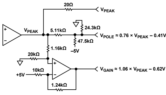
Figure 24. Deriving V_{POLE} and V_{GAIN} from V_{PEAK} With Low-Z Source for Coaxial Cable
