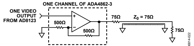
Figure 26. Using ADA4862-3 on AD8123 Outputs
