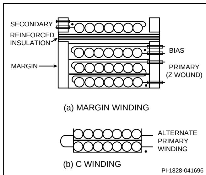
Figure 2. Margin Wound Transformer Cross Section.
