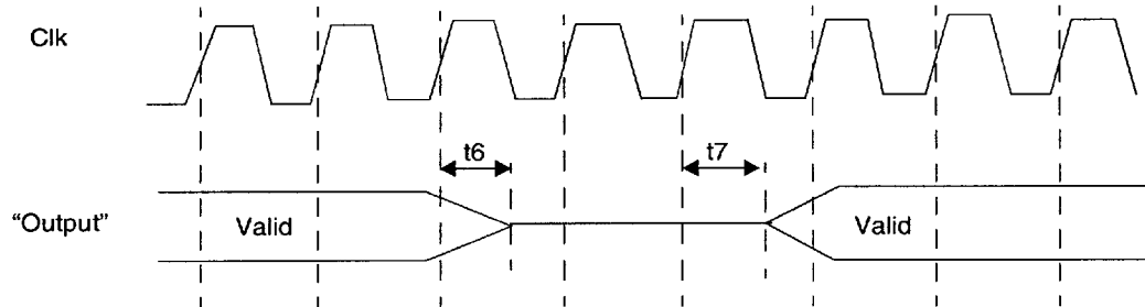
Output Float and Drive Delay
