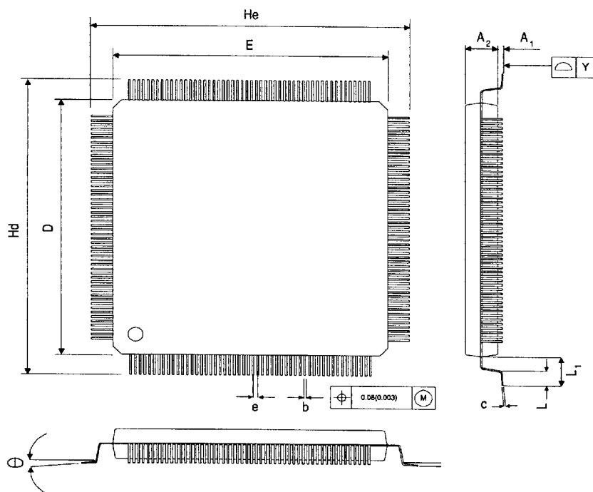
208 LEAD PQFP PACKAGE OUTLINE
