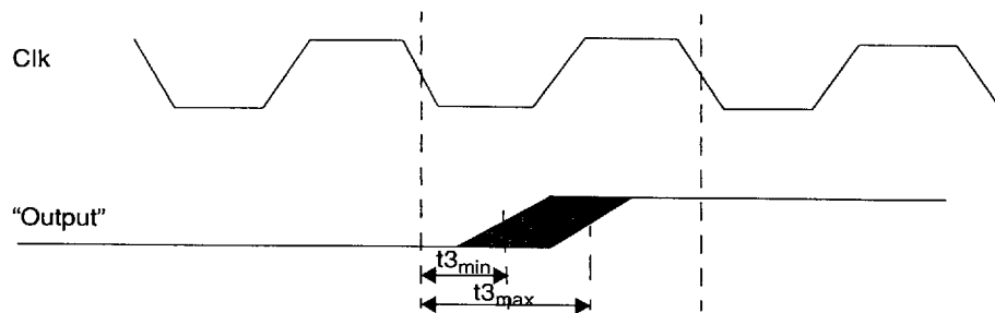
Output Delay from Clock Falling Edge
