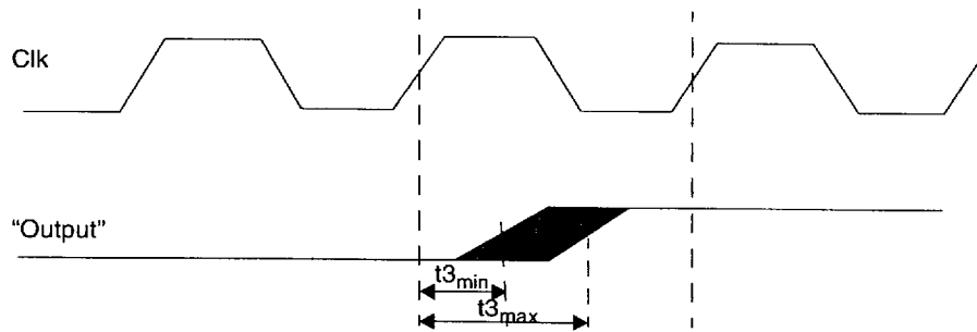
Output Delay from Clock Rising Edge
