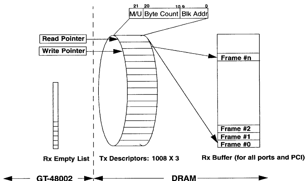
Figure 2 - GT-48002 Buffers and Queues
