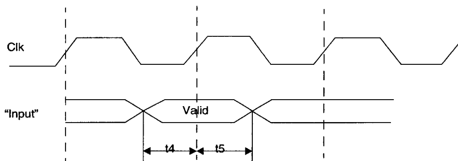
Inputs Setup and Hold
