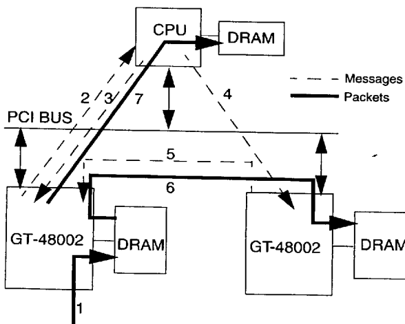
Figure 5 - Unicast Packet Transfer With Intervention
