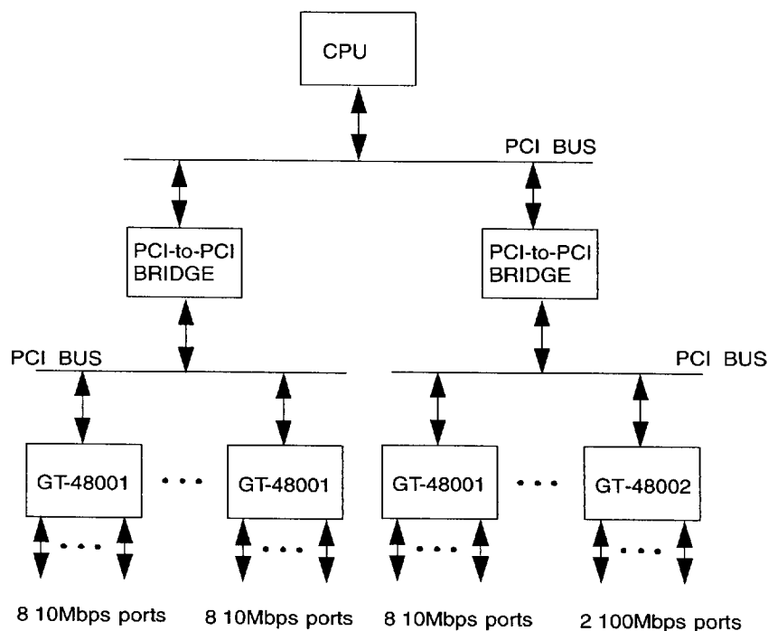
Figure 6 - Switch Expansion
