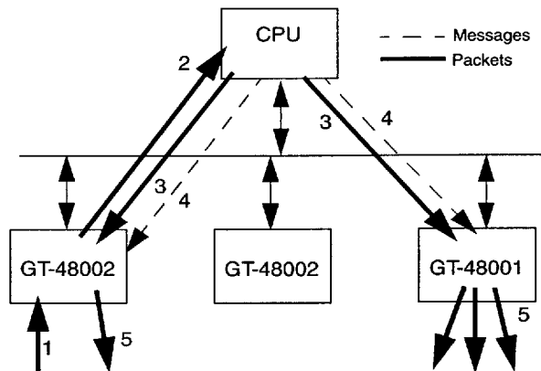
Figure 4 - Multicast Packet Transfer With Intervention
