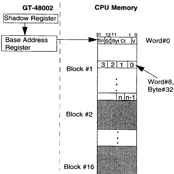
Figure 3 - CPU Data Structure
