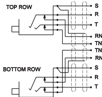
NORMALS OUT
