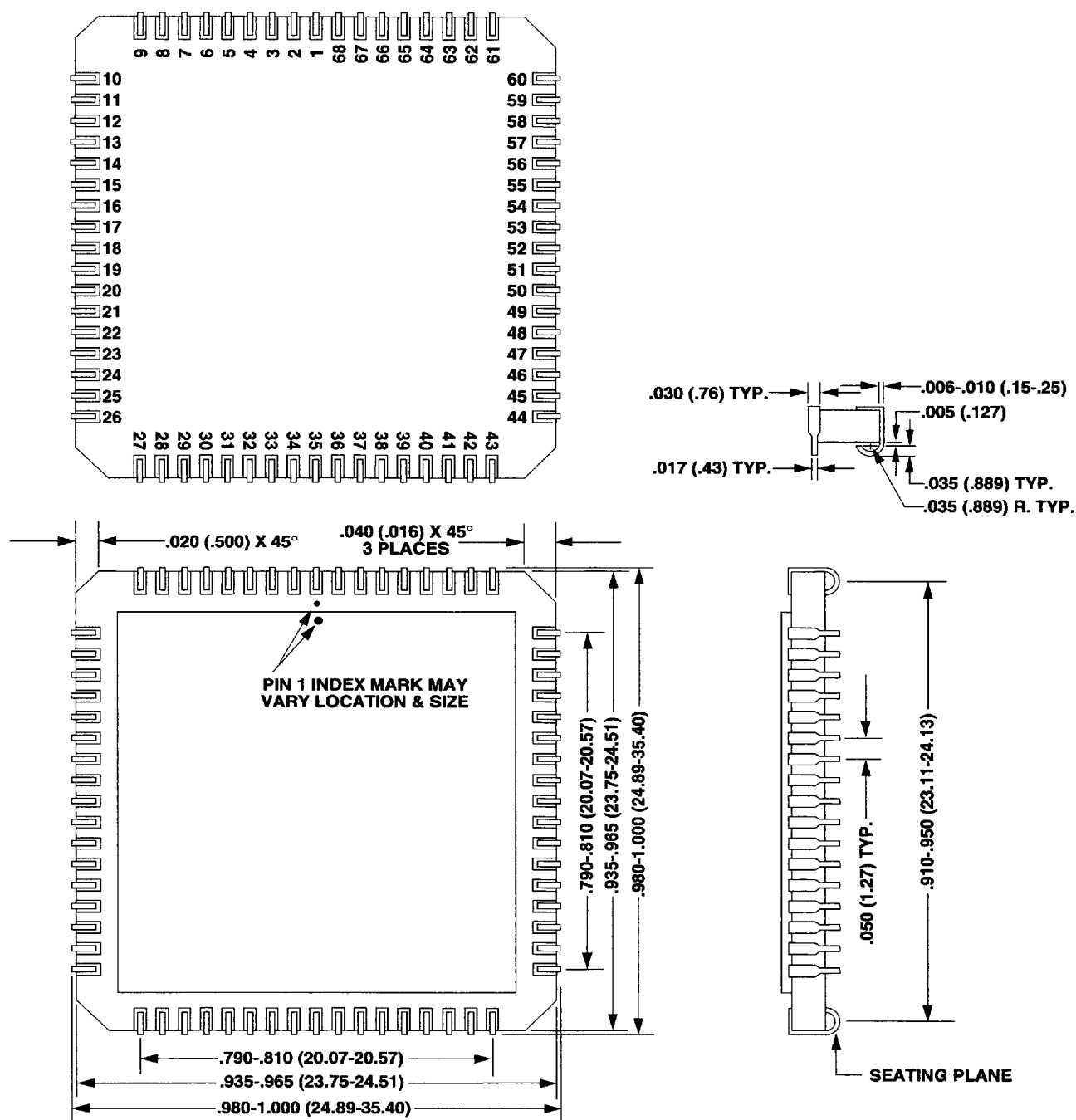
Figure 16. CLDCC Packaging
