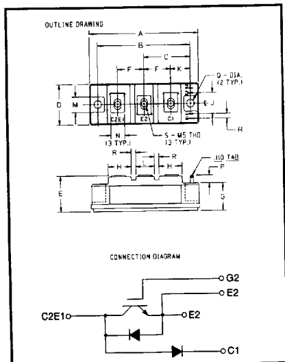
CM100E3Y-12E Outline Drawing
